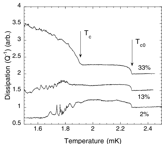
FIG. 3. Dissipation versus temperature for different ^3\text{He} - ^4\text{He} mixtures in aerogel. The ^4\text{He} fraction for the curves (shifted vertically for clarity) are shown along side.
