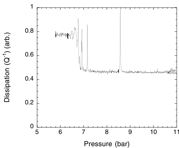
FIG. 2. Q^{-1} versus pressure at 0.3 mK for pure ^3\text{He} in aerogel. At low pressures the ^3\text{He} is in the normal state. The Q^{-1} decreases above 6.7 bar in the superfluid. Sharp peaks mark where the “slow mode” harmonics cross the \approx 790 Hz torsion oscillator frequency (see text) and are not relevant here.
