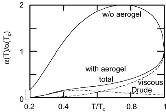
FIG. 1. The calculated transverse sound attenuation vs T/T_c . The attenuation (with aerogel: total) decreases sharply at T_c . The dominant contribution to the attenuation (“viscous”) shows a strong decrease at T_c . The elastic contribution (“Drude”) shows a slow increase originating in the square of the inverse BQP group velocity. Also shown is the behavior of the attenuation in the absence of aerogel, i.e., the limiting behavior if the ^4\text{He} eliminates elastic scattering.
