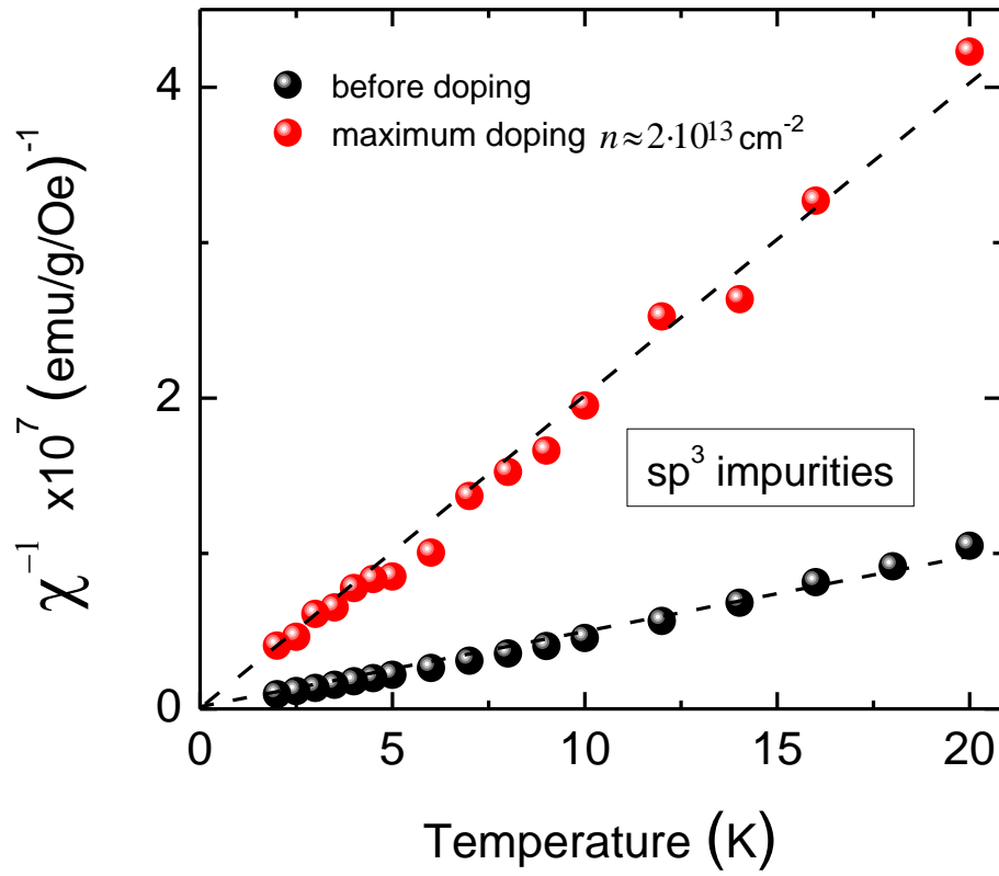
Supplementary Figure S4. Absence of deviations from the Curie law for graphene with \text{sp}^3 impurities. Inverse paramagnetic susceptibility for a sample containing \text{sp}^3 impurities. This sample was heat-treated at 350^\circ\text{C} (see main text). Measurements were done in parallel field H = 5 \text{ kOe} . Constant diamagnetic background subtracted.
