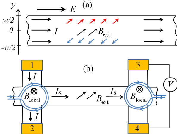
FIG. 2 (color online). (a) Schematic for spin accumulation in the SHE regime. An electric current in a graphene strip drives transverse spin current, resulting in spin density buildup across the strip, Eq. (3). (b) Generation and detection of spin current in the H geometry. Electric current passed through the region of local magnetic field drives spin current along the strip. Voltage generated via inverse SHE is detected using probes 3 and 4. Hanle-type oscillation due to spin precession can be induced by external magnetic field applied in plane.
