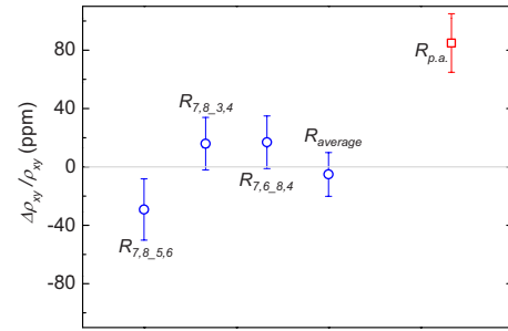
FIG. 4. (Color online) Deviations from quantization in ppm measured with the CCC ( I_{sd}=1.5 \mu\text{A} ) for different contact configurations and their average (blue circles). The red square ( R_{p,a} ) represents the deviation for a poorly annealed sample at a source-drain current of 0.5 \mu\text{A} .
